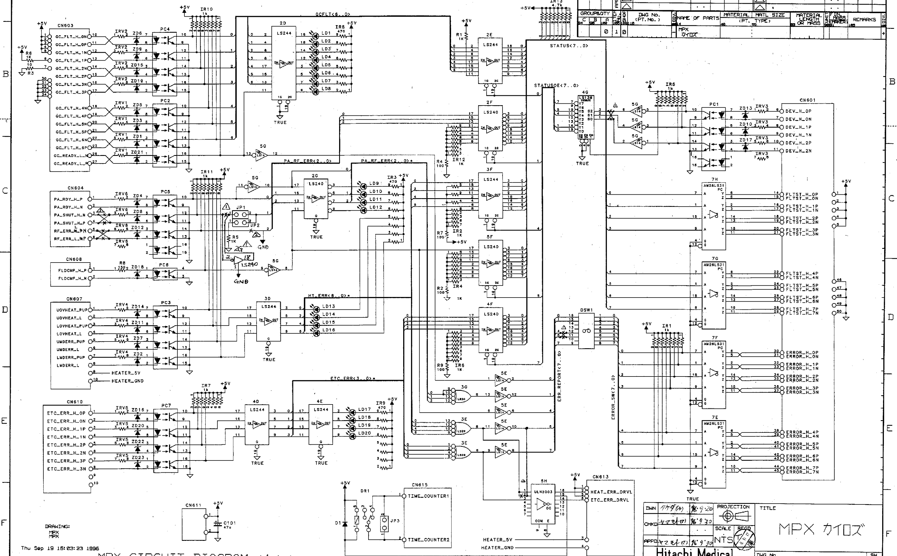
MPX CIRCUIT DIAGRAM (1/2)
