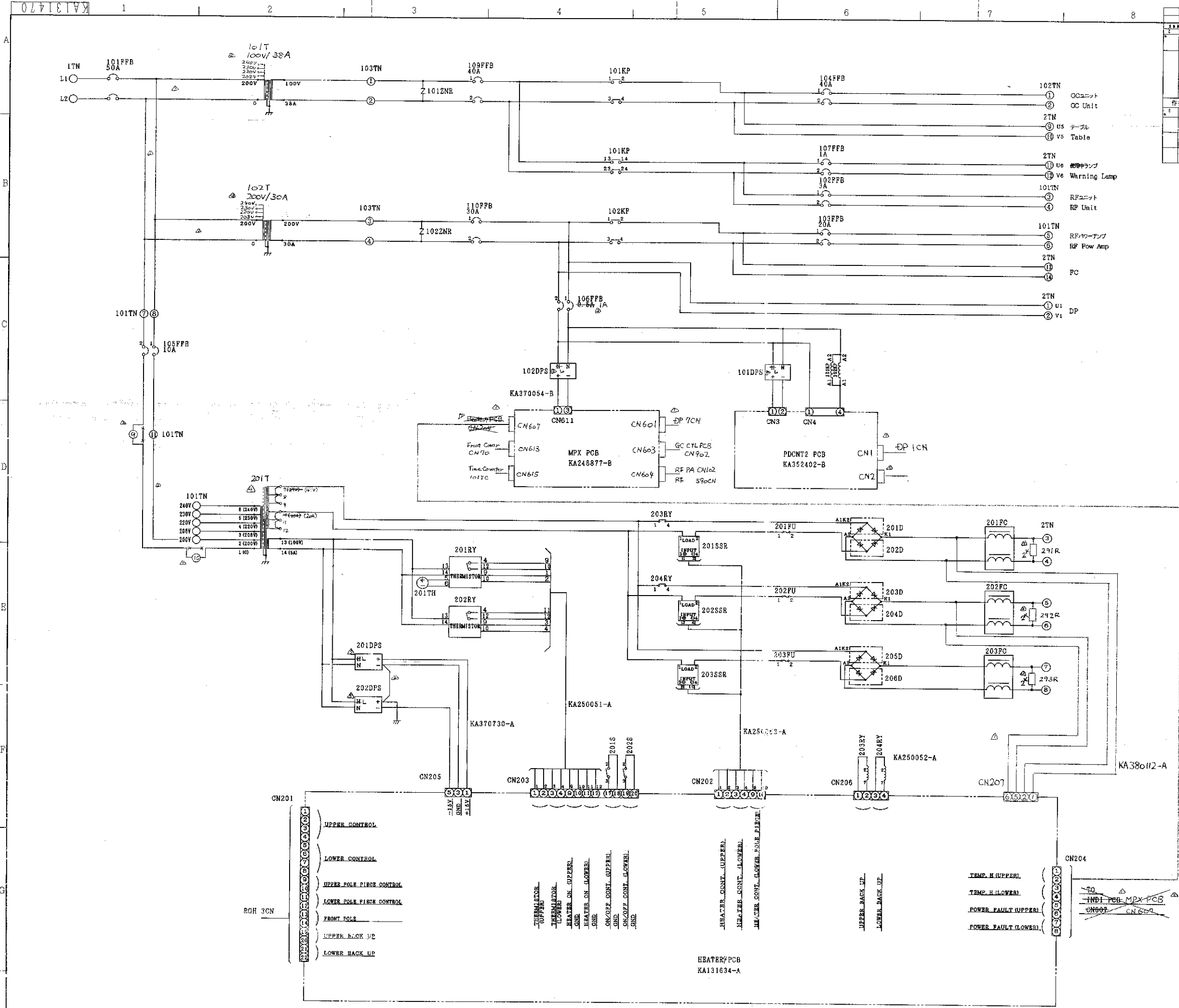
PD Heater Circuit Diagram
