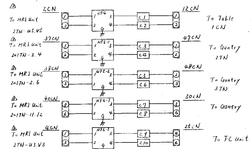
△ MR-FB-4A circuit diagram
